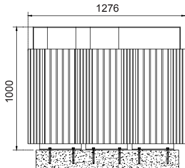
DTS-HXB-09-PS-01 FRONT VIEW
