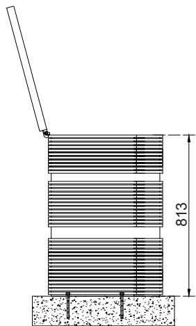
FRONT VIEW DOOR OPENING
