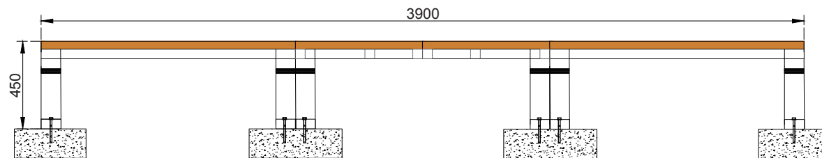
FRONT VIEW
